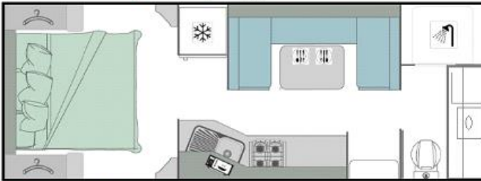
22'6" Rear club (Trackvan)
