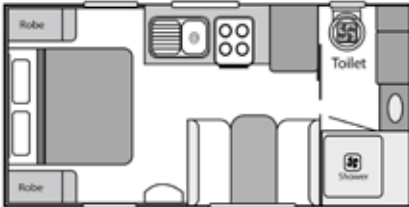
17'6 ROADSIDE KITCHEN SINGLE AXLE
